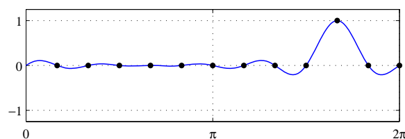
Fig. 7.1 Any set of data at equispaced points can be interpolated by a trigonometric polynomial, and if the trapezoidal rule is applied to the data, the result I_N is equal to the integral of the interpolant. Here the data correspond to a Kronecker delta function on a grid with N = 12 , the interpolant is a periodic sinc function, and the integral is equal to h = 2\pi/N . Interpolants to more general data can be regarded as linear combinations of translates of such periodic sinc functions. Analogous observations hold for the trapezoidal rule on the unit circle or the real line.
